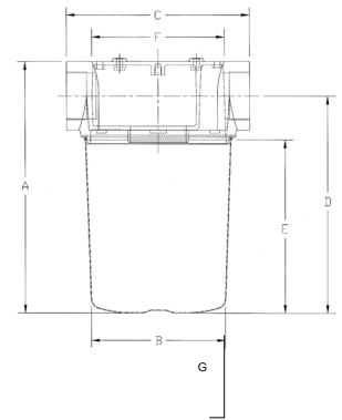
Dimension tolerance \pm 1/4"
